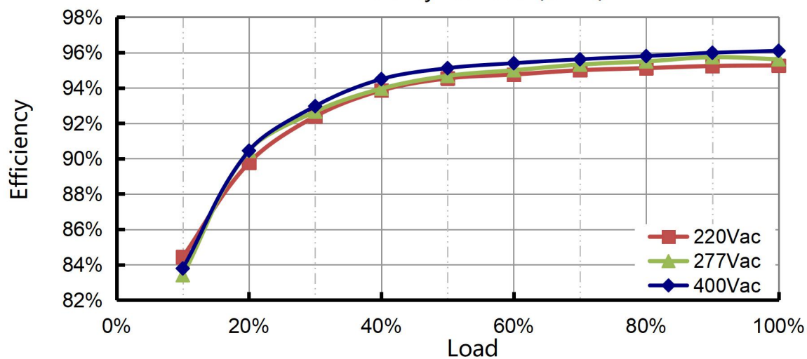
Efficiency vs. Load (C240)
