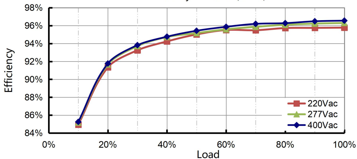
Efficiency vs. Load (C210)
